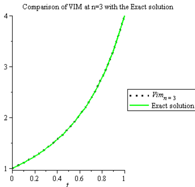
Fig 1. Plots comparing VIM approximate solution at n=3 with the Exact solution
