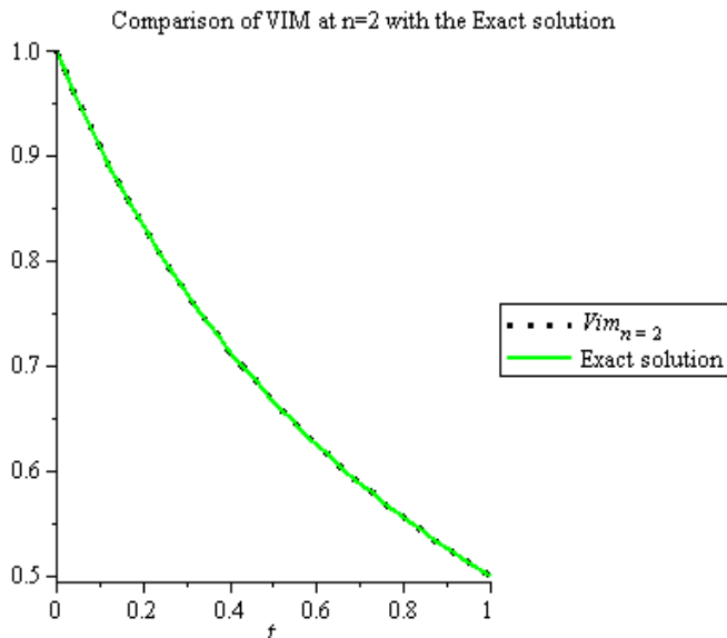
Fig 1. Plots comparing VIM approximate solution at n=2 with the Exact solution
